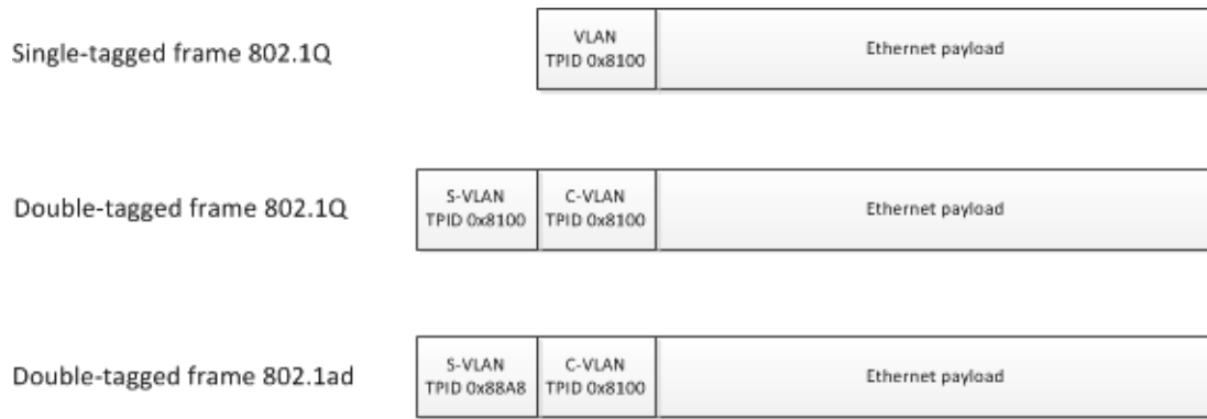
Figure 1 – Single and double tagged Ethernet frames Note: This figure is provided for illustrative purposes only
